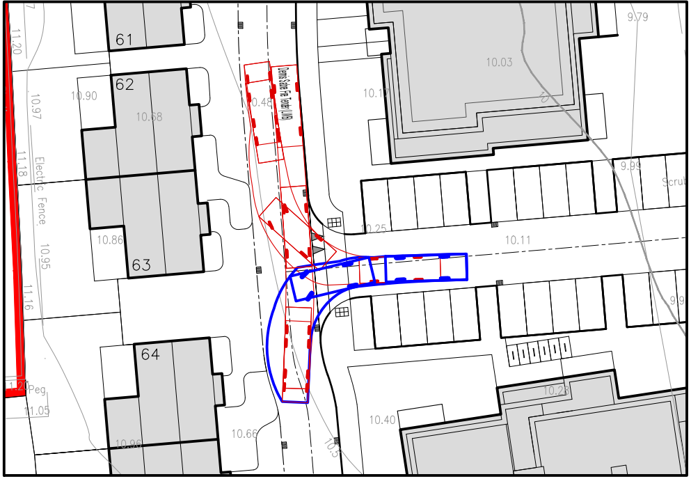
INSERT C SCALE 1:500
